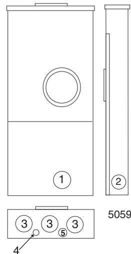
320 AMP-4 OR 5 TERMINAL - METER MAIN WITH BREAKERS - 1Ø3W - RINGLESS - 120/240 VAC
