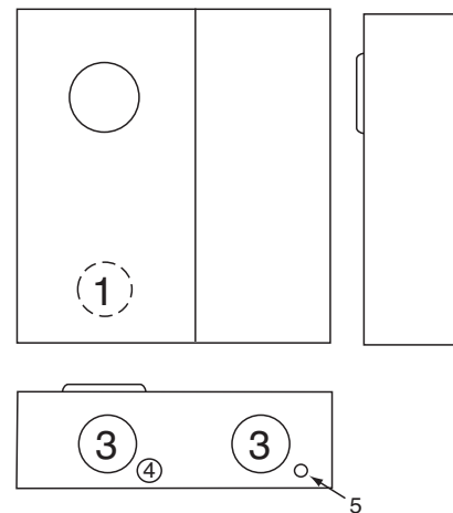
320 AMP METER SOCKET – 1Ø3W – RING TYPE – 600 VAC
