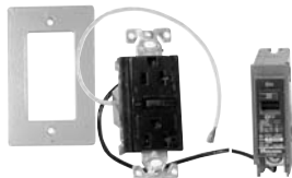
K5400-520GR 20 amp 120V GFI receptacle and circuit breaker kit
