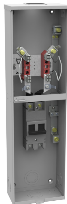
U7607-RL-200-KK-CECHA SUPPLIED WITH 200 AMP CIRCUIT BREAKER
