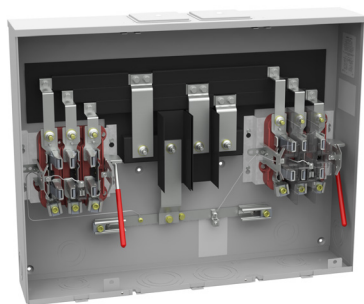
U2732-XT-PED (shown without pedestal)
