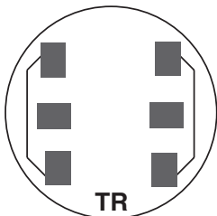
3-WIRE FORM 4S WITH BYPASS
