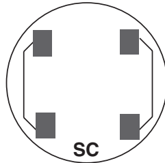
2 and 3-WIRE FORMS 1S & 2S with BYPASS
