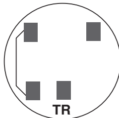
2-WIRE FORM 3S with BYPASS
