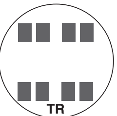
2 ELEMENT 2Ø3W, 2Ø4W, 3Ø3W FORM 5S
