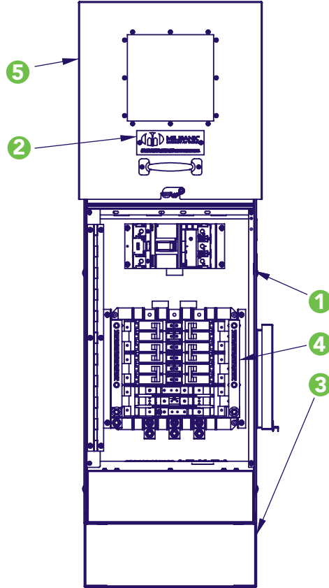
Front View, w/out Deadfront
