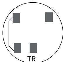
2-WIRE FORMS 3S with bypass
